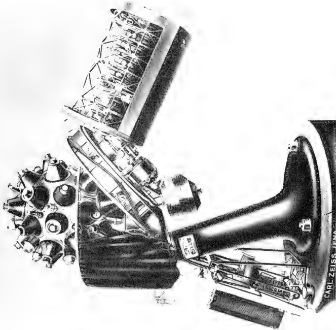
1. Projection apparatus of the Carl Zeiss Jena Planetarium.
