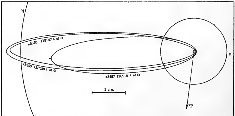
FIGURE 7.—The orbits of three \delta -Aquadrid meteors ( q=0.07 A. U.)
