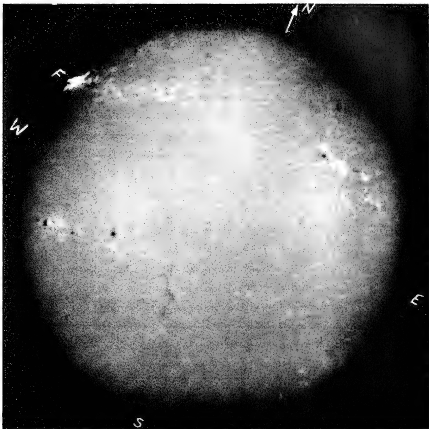
The sun in H\alpha light showing the great flare of February 23, 1956. Photograph courtesy of Kodaikanal Observatory, India.
