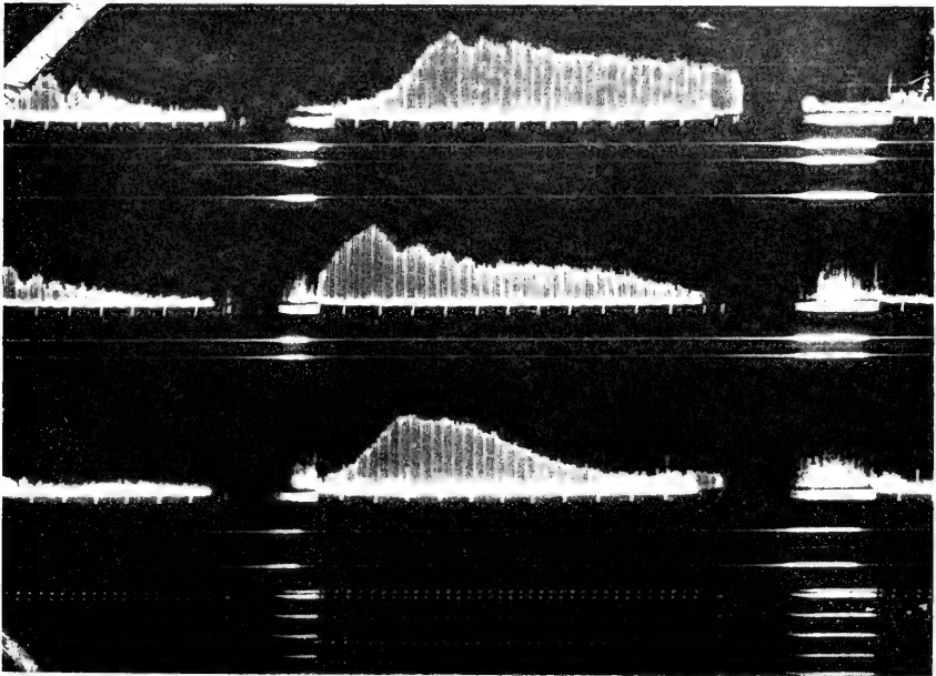
2. Record of radio pulses from a meteor. (J. G. Davies, Jodrell Bank, England.)
