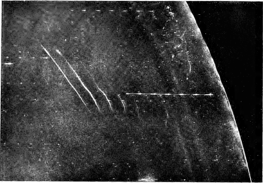
1. A persistent meteor train. Multiple photographs at the intervals of 2 seconds show the fading and distortion. (J. R. Coultis.)
