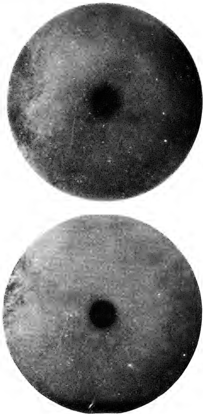
Two photographs of a Perseid shower made simultaneously from two stations in New Mexico
