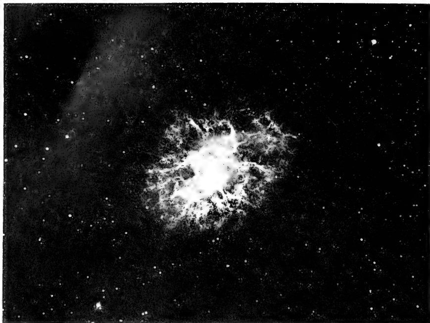
2. The Crab nebula photographed in hydrogen light. (Photograph by permission of Mount Wilson and Palomar Observatories.)
