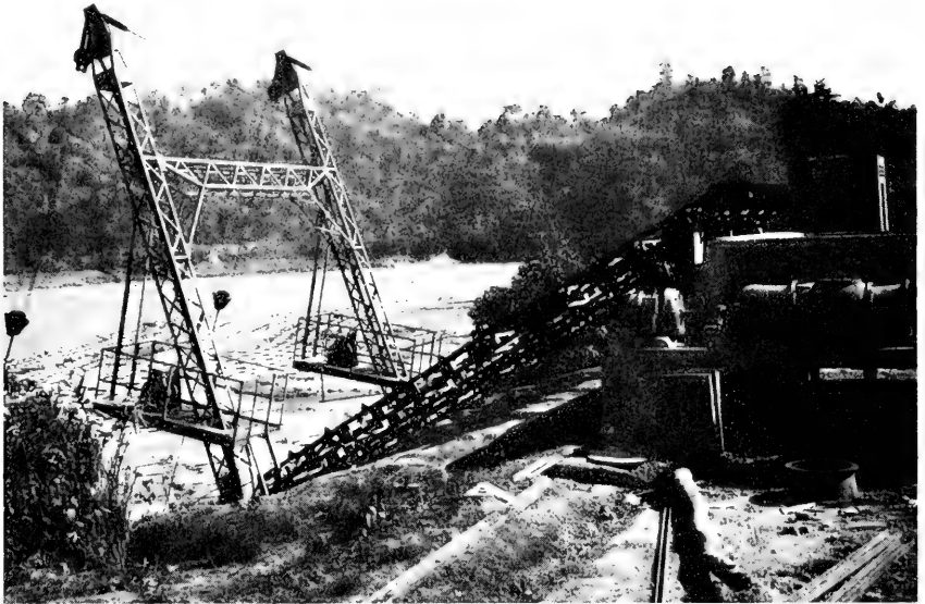
1. At the recently completed Karnaphuli Paper Mill, East Pakistan, bamboo will be used to produce 100 tons of pulp per day. Equipment shown was specially designed to lift rafted bundles of bamboo from the river to the flume, by way of which they will reach the mill.
