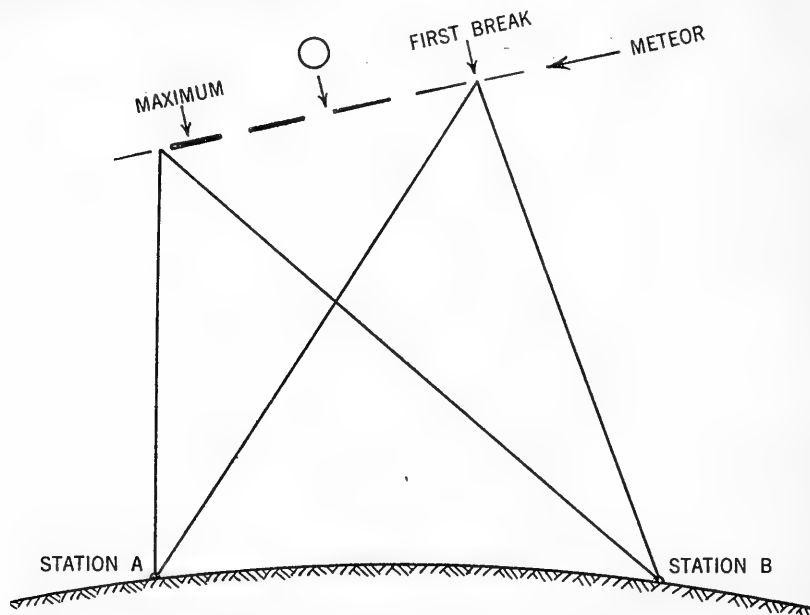
FIGURE 3.—Diagram showing a meteor photographed simultaneously from stations A and B; the circle represents a common point on both photographs of the trail.
