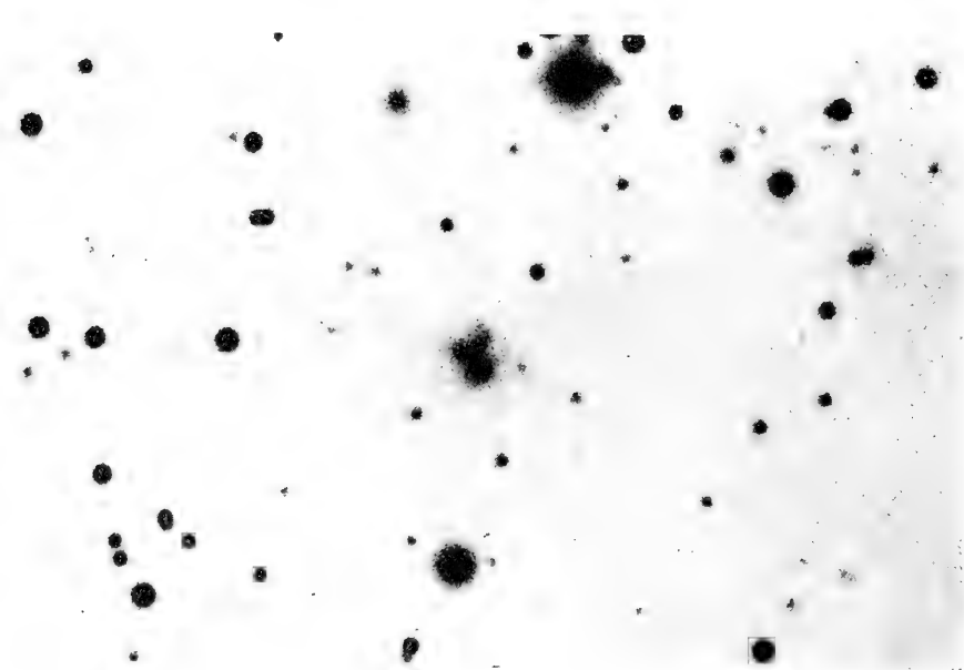
1. Galaxies in collision. (Photograph by permission of Mount Wilson and Palomar Observatories.)
