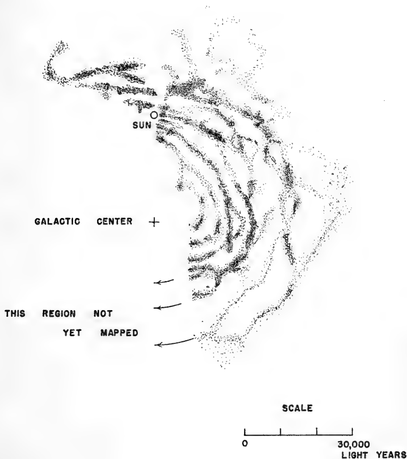
FIGURE 4.—Spiral structure of the local galaxy. (Reproduced by permission of G. Westenhout and M. Schmidt, Leiden, Holland.)
