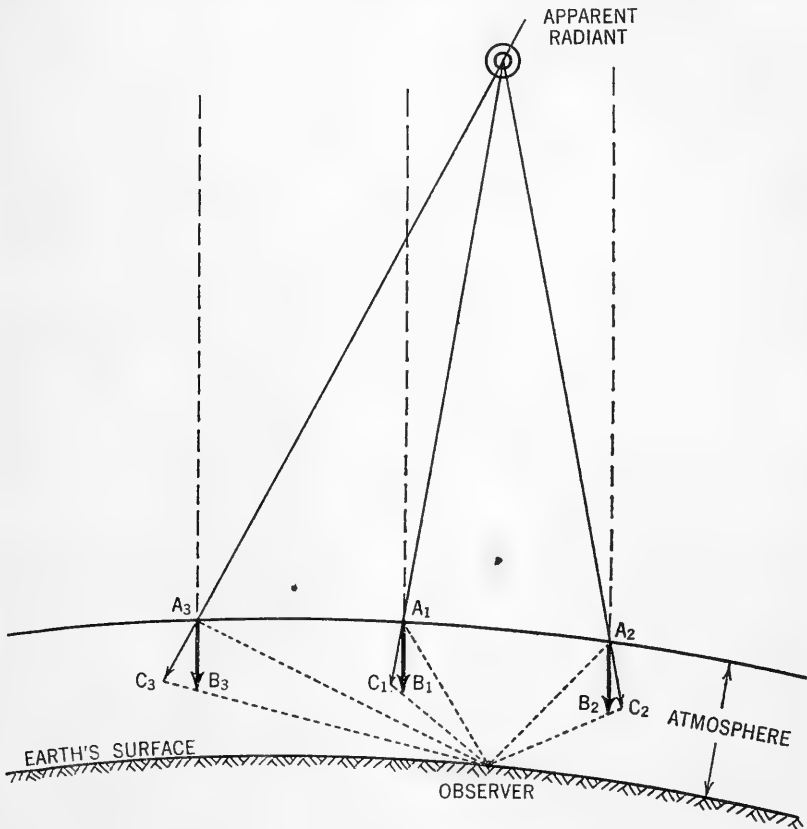
FIGURE 2.—Trails and radiant of a meteor shower. Above the atmosphere the parallel dashed lines show the real paths of the meteors A_1 , A_2 , and A_3 ; solid lines show their apparent paths. In the atmosphere the arrows AB show the real meteor paths, and the arrows AC show the paths as they appear to the observer.
