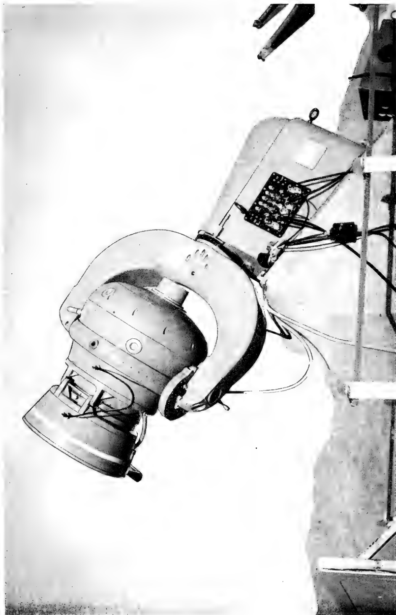
The Baker Super-Schmidt meteor camera.
