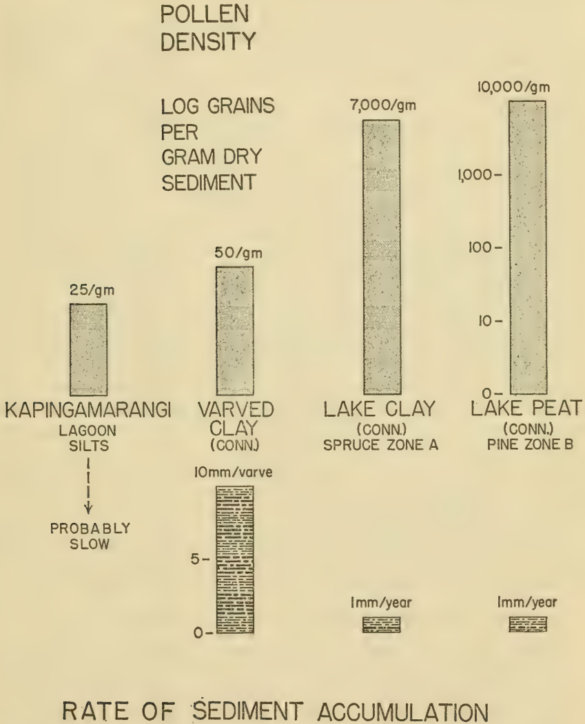
FIGURE 5.—Pollen density in sediments compared with the rate of sediment accumulation. Kapingamarangi lagoon sediments (left) are low in pollen, owing to poorly developed local vegetation; the varved clay (second from left) is low in pollen because of dilution of pollen rain by rapid sedimentation; the sediments in the two remaining examples (right) are rich in pollen because of dense contributing vegetation combined with a slow sedimentation rate.
