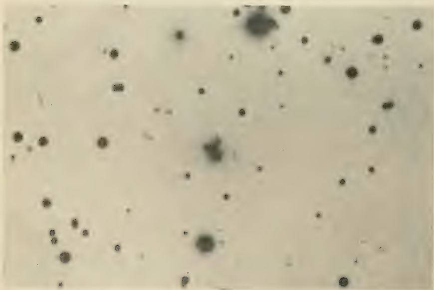
1. Galaxies in collision. (Photograph by permission of Mount Wilson and Palomar Observatories.)
