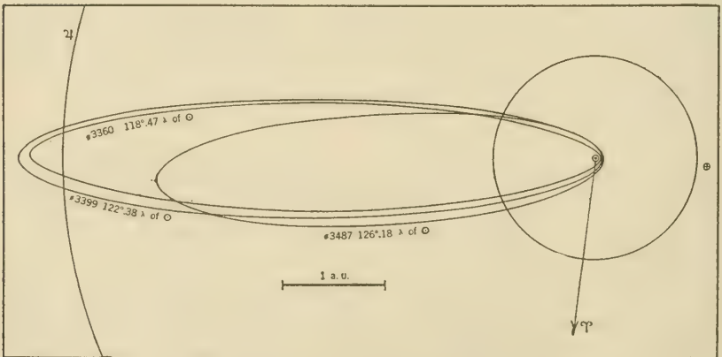
FIGURE 7.—The orbits of three \delta -Aquadid meteors ( q=0.07 A. U.)
