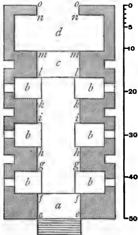
FIG. 1. OUTER GATEWAY.
